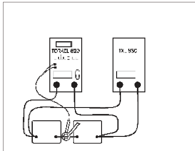
TORQUEL 820 and the extra load TXL 830
